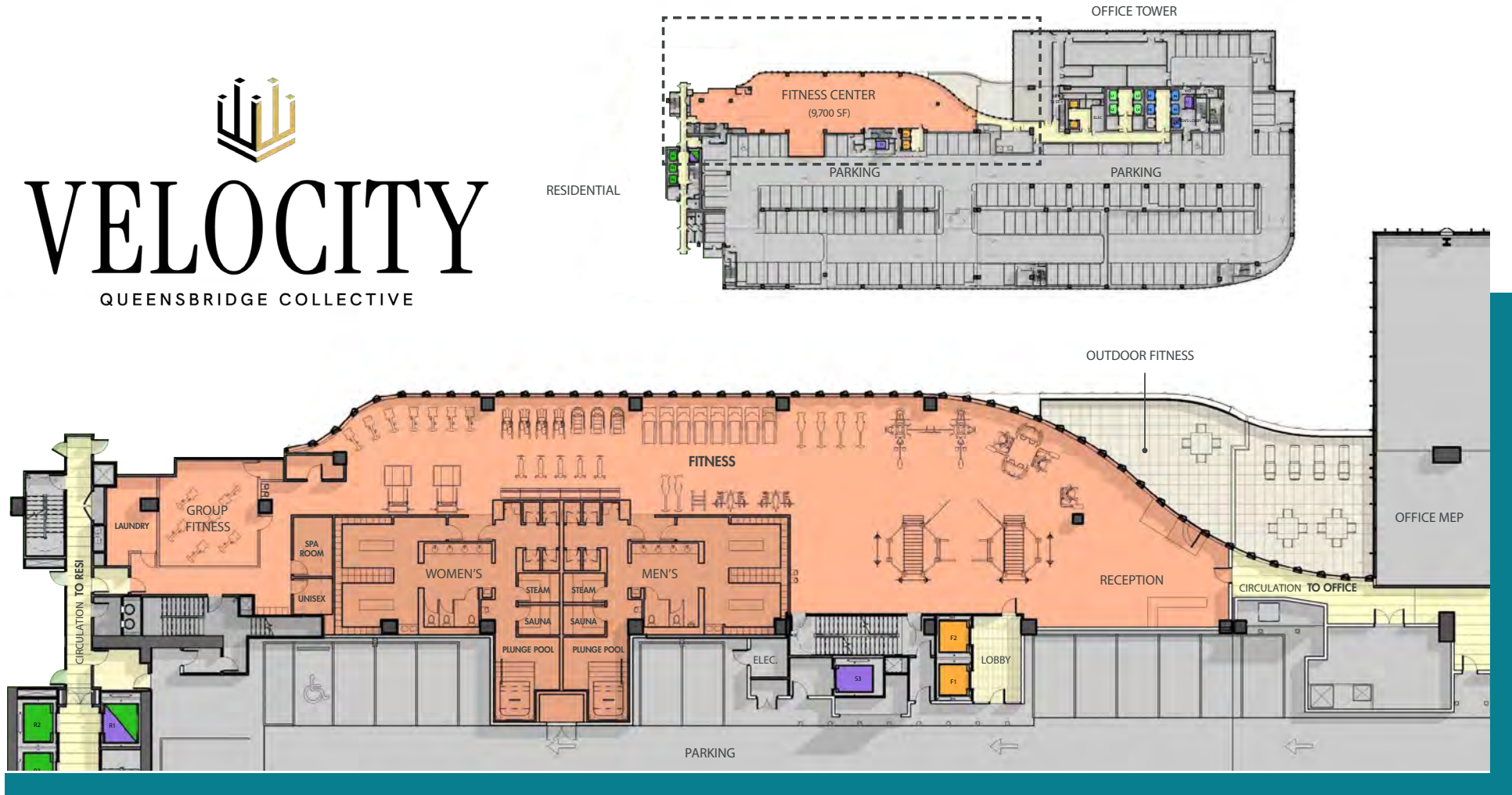
L9 FLOOR PLAN - FITNESS CENTER
